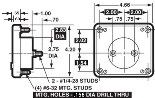
4-1/2" Model 29 & 29T, 49, 59, & 89
